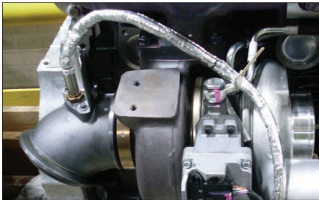
With the advent of SCR technology there is no longer a NO x catalyst in the exhaust aftertreatment. Therefore, the NO x sensor has been moved to the turbocharger downpipe.
