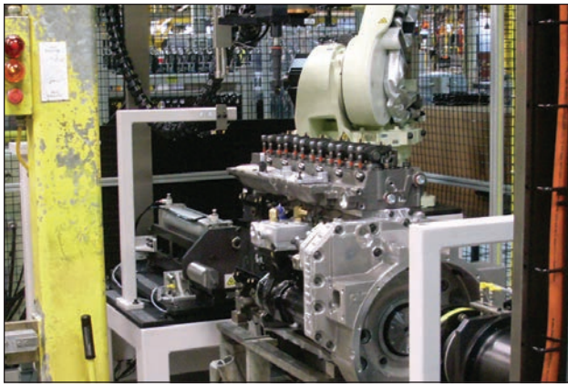
For the 2013 consumer pickup trucks, the cylinder head was revised. Here is a picture of a machine that automatically sets the valve lash of the intake and exhaust valves.
