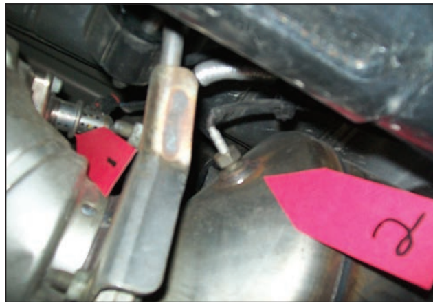
Arrow #1, DEF dosing valve. Arrow #2, EGT3 sensor
